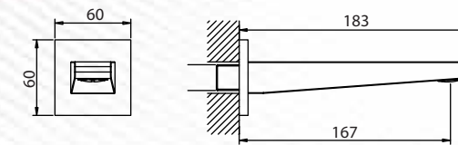
Bath Spout in Polished Chrome Q213100420 MRP: ₹6,490
